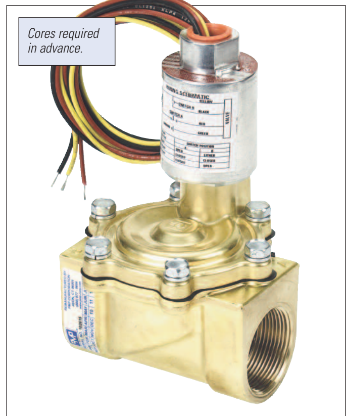
PMP #22058 2-Stage, 1 1/2" Threaded with Coil, 3-Wire MFG #067028
