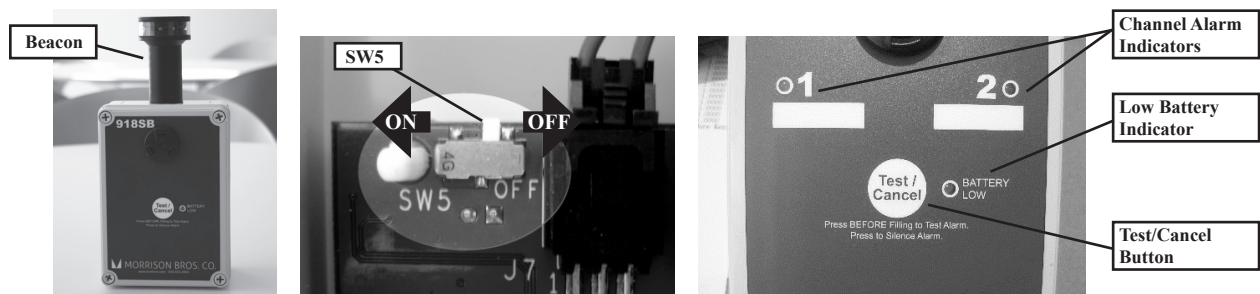
Fig. 1 Alarm with Beacon, Power Switch (SW5), Channel Alarm Indicators, Battery Low Indicator and Test/Cancel Button on the 918DB
