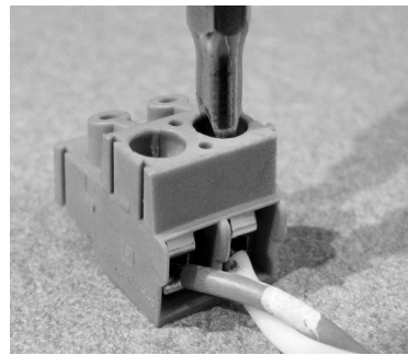
Figure 2 Wiring the Channel Input Connector
