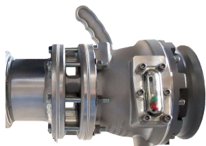
5200-SFI shown mounted on petroleum tank
