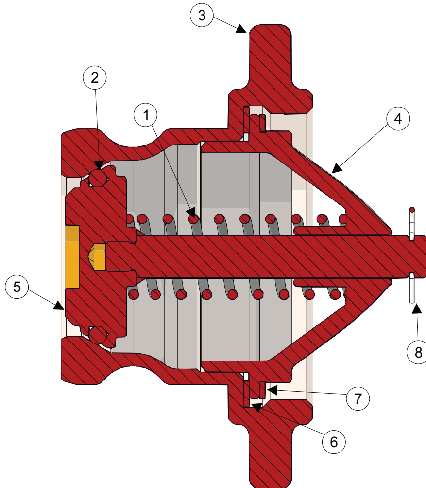
2" x 3" stainless vapor adapter Bill of Materials DBVA73-200
