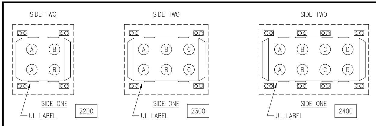
STRAIGHT THRU, ELBOW AND SAUSER SIGHT GLASS
