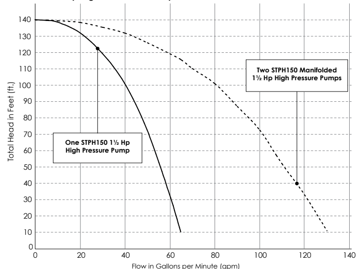
1½ Hp High Pressure Fixed Speed Turbine Performance Chart
